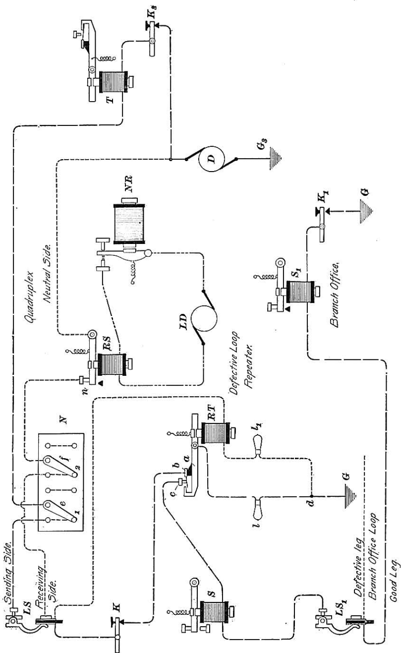
MOFFAT DEFECTIVE-LOOP REPEATER IN WESTERN UNION OFFICES THAT USE DYNAMOS.
